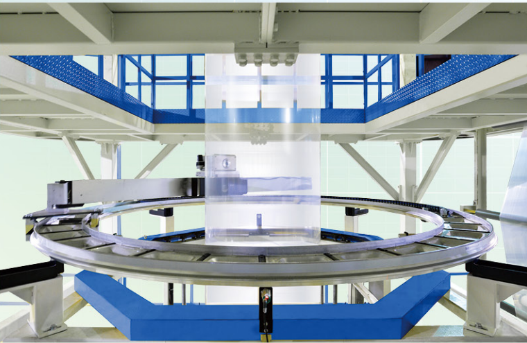
Online film thickness scanner option 可選配線上厚薄偵測系統
